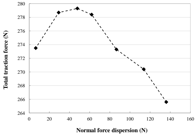
FIGURE 2. Variation of total traction force with load dispersion
