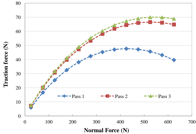
FIGURE 1. Relation between normal and tangential force for different number of wheel passage
